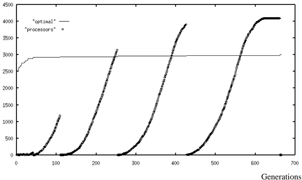
Figure 14. The Number of Processors which contain the best chromosome using the mpdGA to optimize the order 4 fully deceptive problem, interleaved. Also plotted is the best value * 10, for comparison. The sudden drops in the number of processors used, represent a new best solution found in one of the processors.
