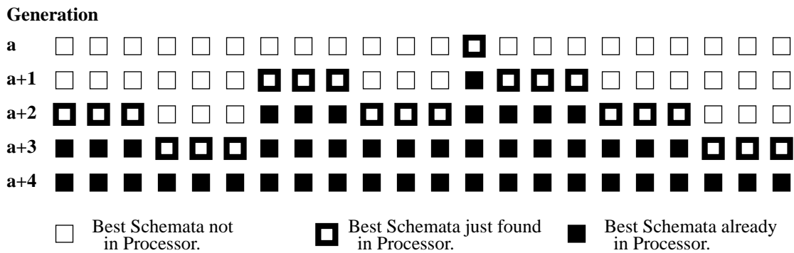
Figure 6. Making the large assumption that the best schemata is not lost during crossover or mutation, the above diagram depicts how the schemata could spread through the processors, using mdpGA configuration #3.
