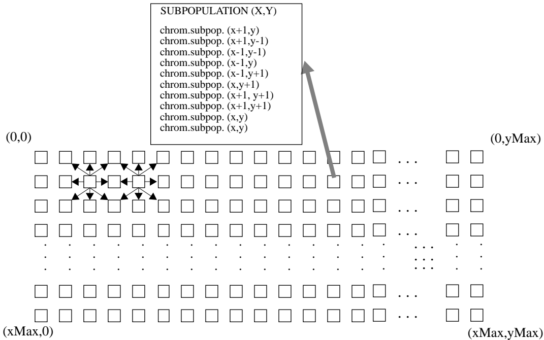
Figure 4. The architecture of subpopulations, arrangement #2. A two dimensional array of processors is assumed. Each processor contributes one of its two chromosomes to each of its 8 nearest neighbors. A sample population for processor (x,y) is shown. The processors are connected in a toroid.
